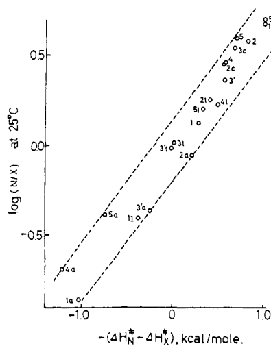
Figure 1. Plots of \log(N/X) vs. -(\Delta H_N^\ddagger - \Delta H_X^\ddagger) for the Diels-Alder reactions of cyclopentadiene with various methyl-substituted dienophiles at 25°. Numbers are the same as those in Table I.
